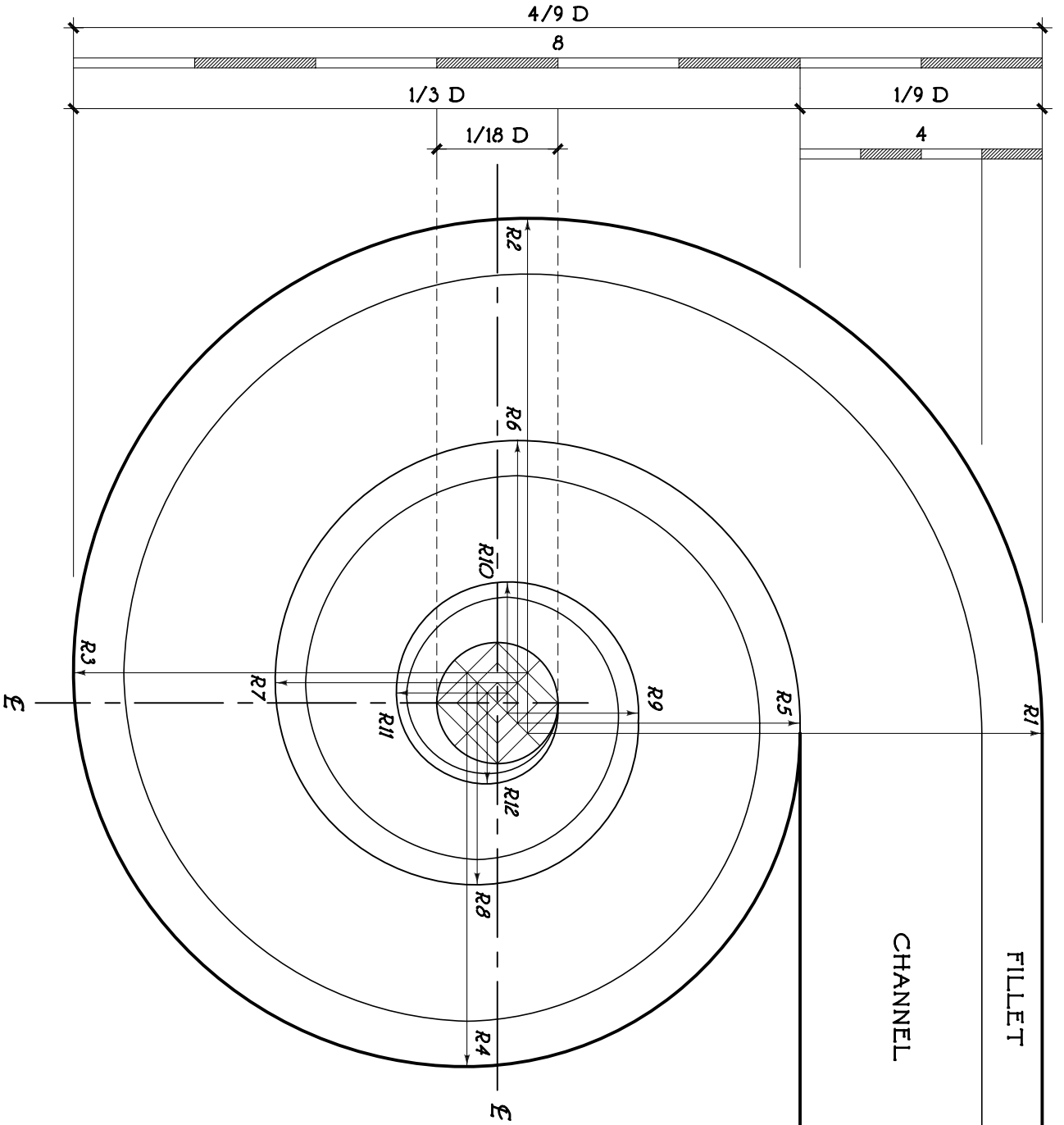
THE EYE DIAGRAM
